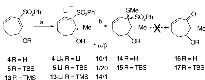
Scheme 2. Initial sulfenylation attempts. a) MeLi, THF, –78 °C, b) Me 2 S. TMS = trimethylsilyl.
