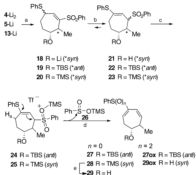
Scheme 3. γ-Sulfenylation and diene transposition. a) 1. MeLi, THF, –78 °C, 2. Ph 2 S 2 ; b) warm to RT, c) TMSOTf, Et 3 N, CH 2 Cl 2 , d) reflux. RT = room temperature, Tf = trifluoromethanesulfonyl.
